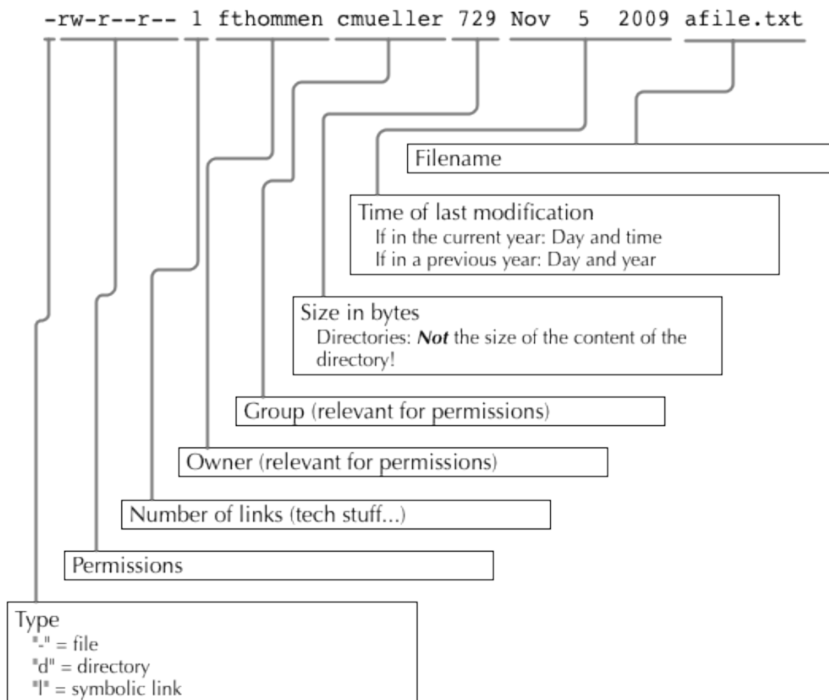
Fig. 3: Elements of a long file listing ( ls -l )
